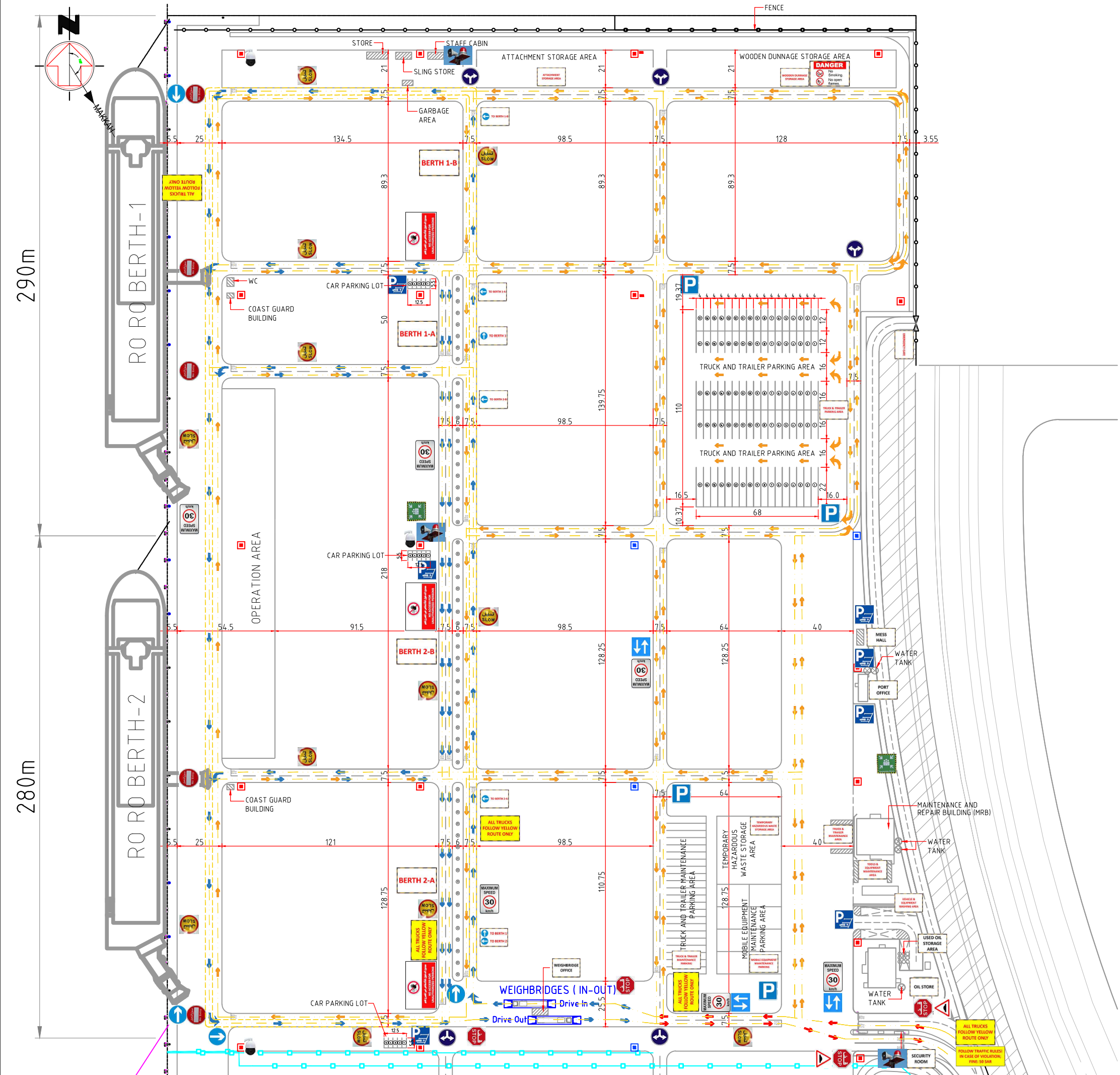
RORO TERMINAL ROAD LAYOUT SCALE: NTS
